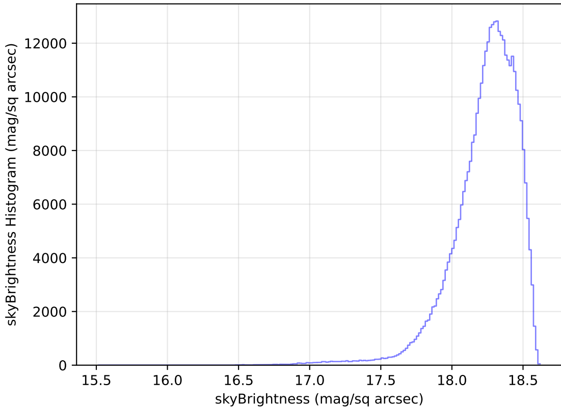
roll_pause_mjdp365_v3.4_10yrs WFD y band: skyBrightness Histogram
