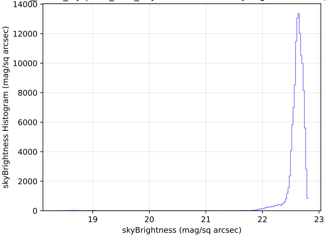
roll_pause_mjdp365_v3.4_10yrs WFD u band: skyBrightness Histogram
