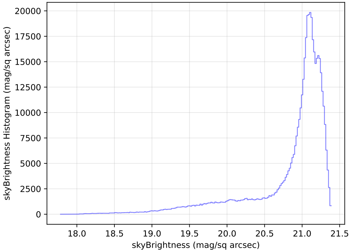
roll_pause_mjdp365_v3.4_10yrs WFD r band: skyBrightness Histogram
