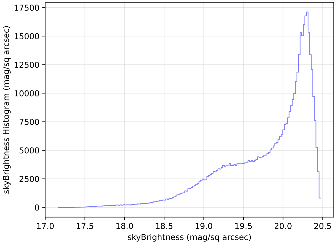
roll_pause_mjdp365_v3.4_10yrs WFD i band: skyBrightness Histogram
