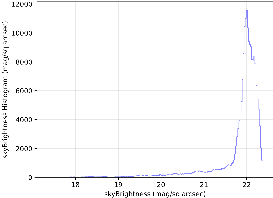
roll_pause_mjdp365_v3.4_10yrs WFD g band: skyBrightness Histogram
