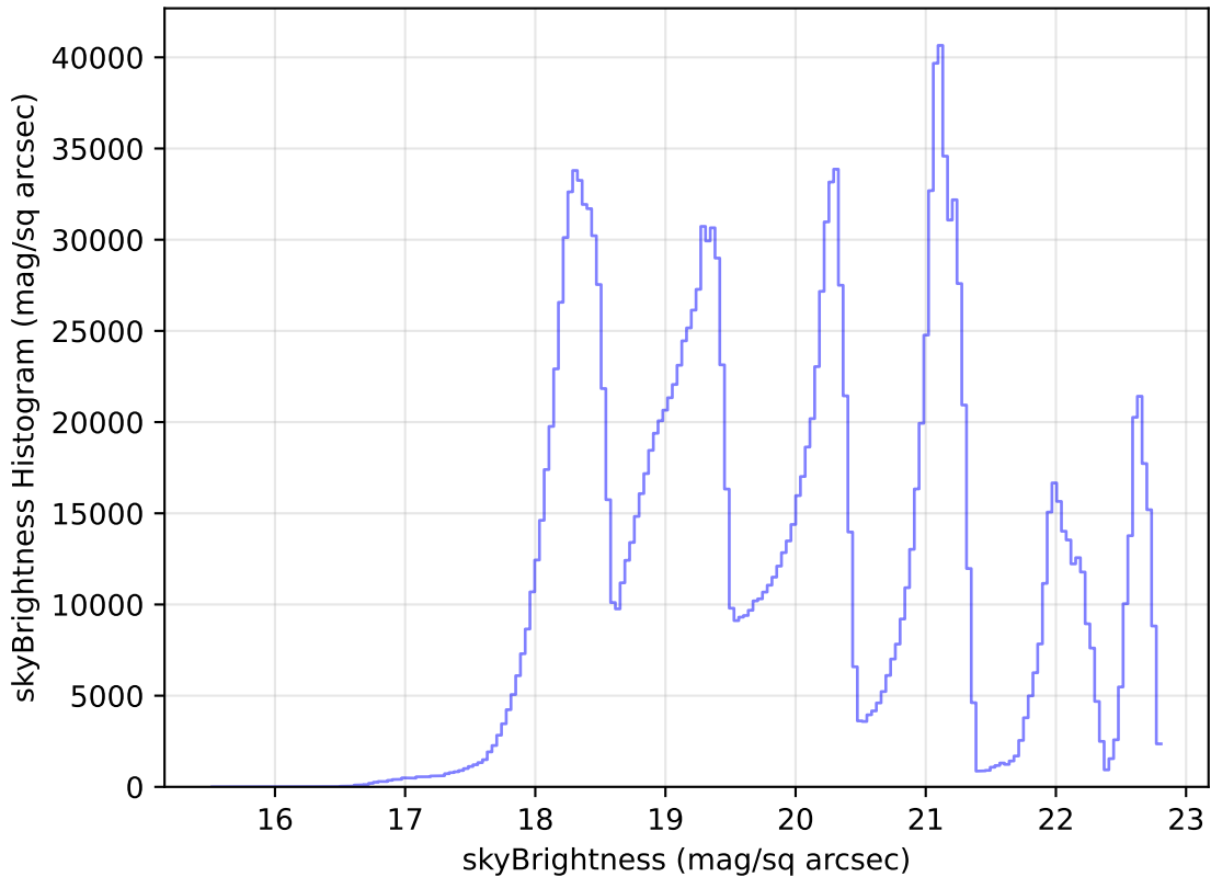
roll_pause_mjdp365_v3.4_10yrs WFD all bands: skyBrightness Histogram
