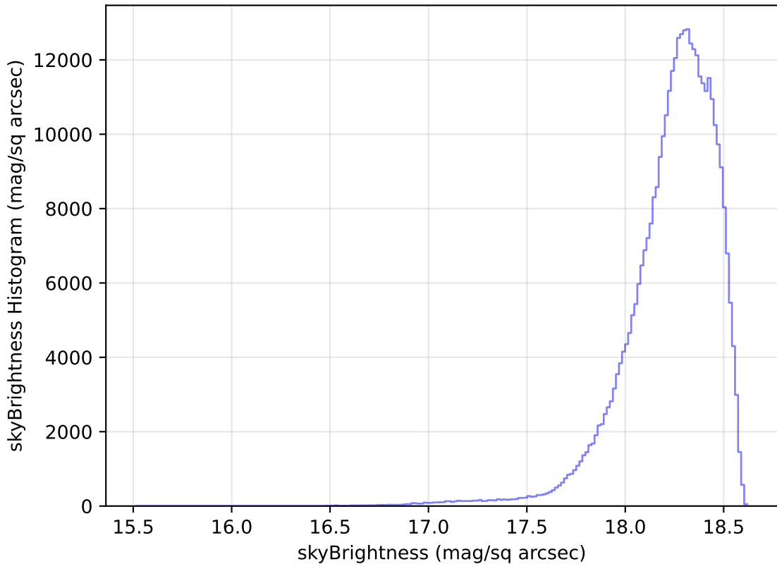
roll_pause_mjdp365_v3.4_10yrs All sky y band: skyBrightness Histogram
