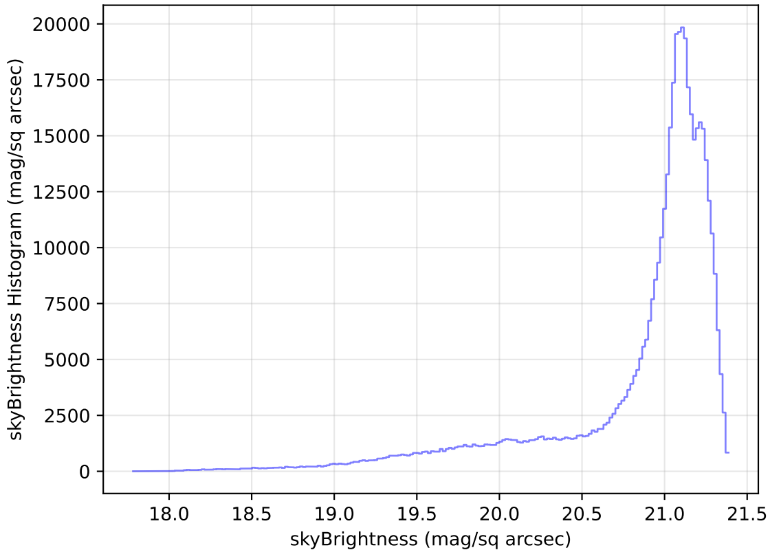
roll_pause_mjdp365_v3.4_10yrs All sky r band: skyBrightness Histogram
