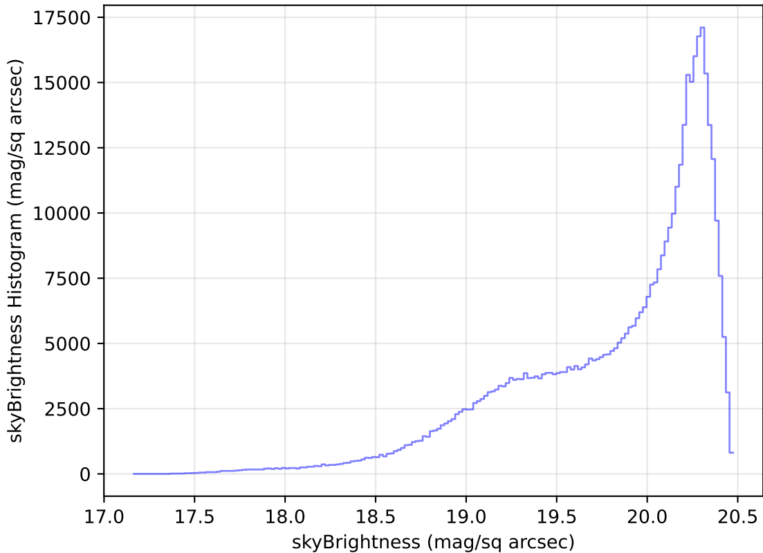
roll_pause_mjdp365_v3.4_10yrs All sky i band: skyBrightness Histogram
