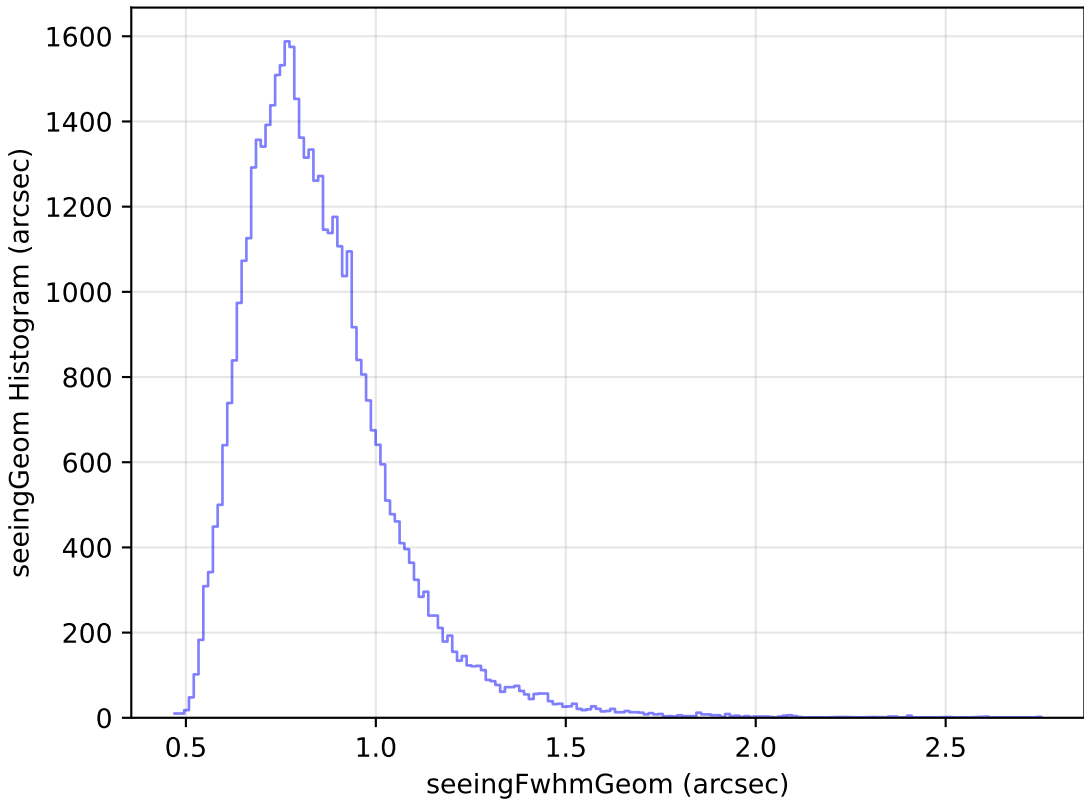
roll_pause_mjdp365_v3.4_10yrs Yr 1 y band: seeingGeom Histogram
