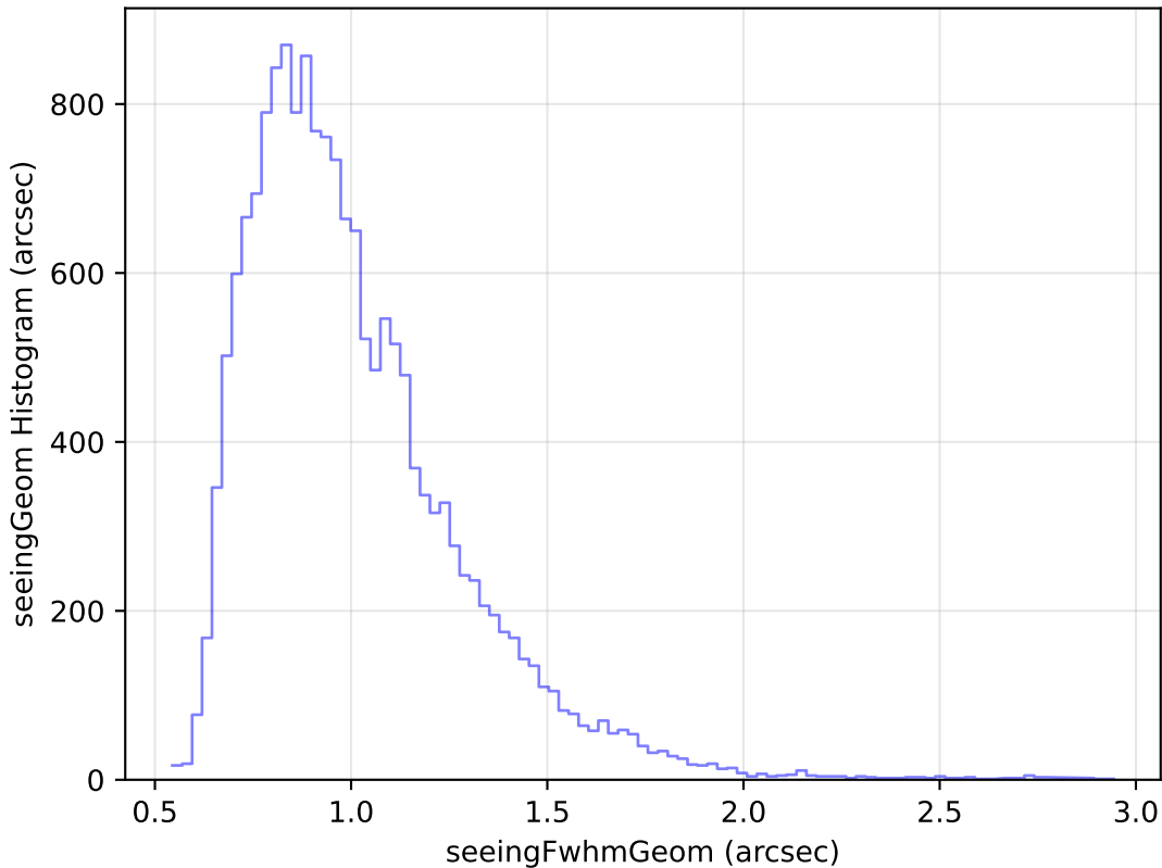
roll_pause_mjdp365_v3.4_10yrs Yr 1 u band: seeingGeom Histogram
