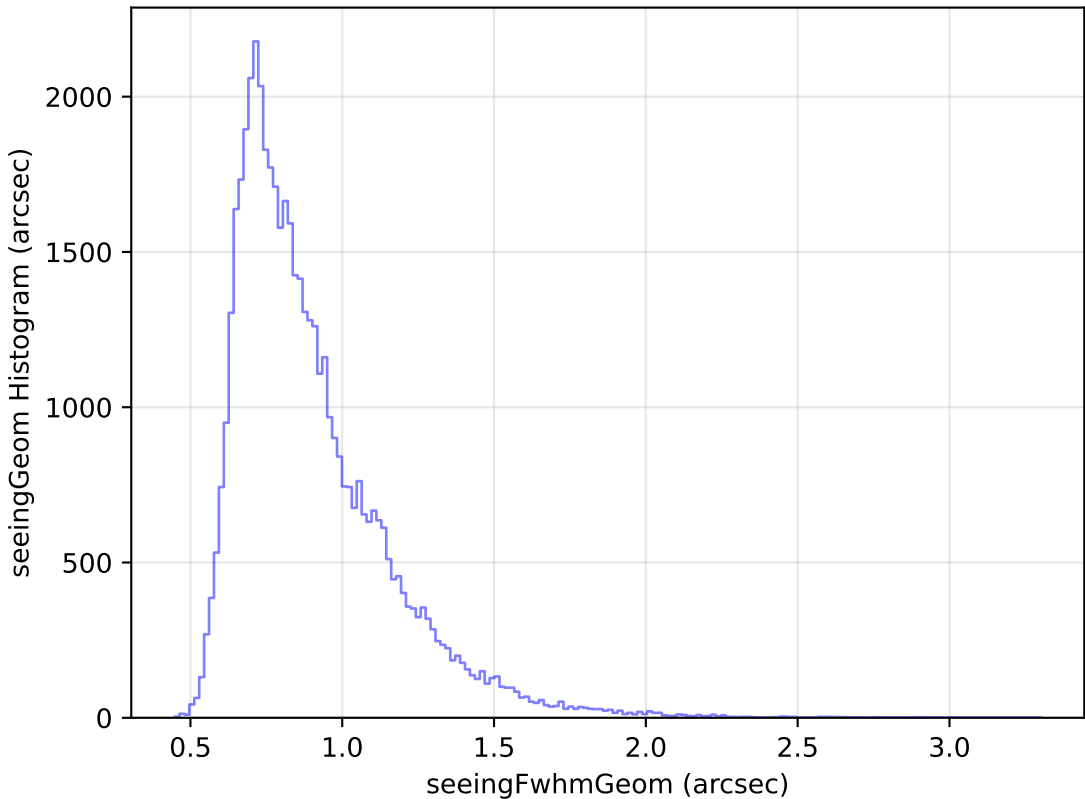
roll_pause_mjdp365_v3.4_10yrs Yr 1 r band: seeingGeom Histogram
