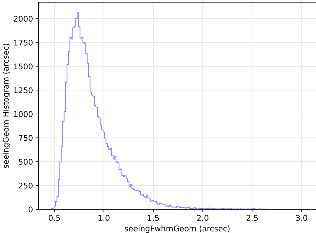
roll_pause_mjdp365_v3.4_10yrs Yr 1 i band: seeingGeom Histogram
