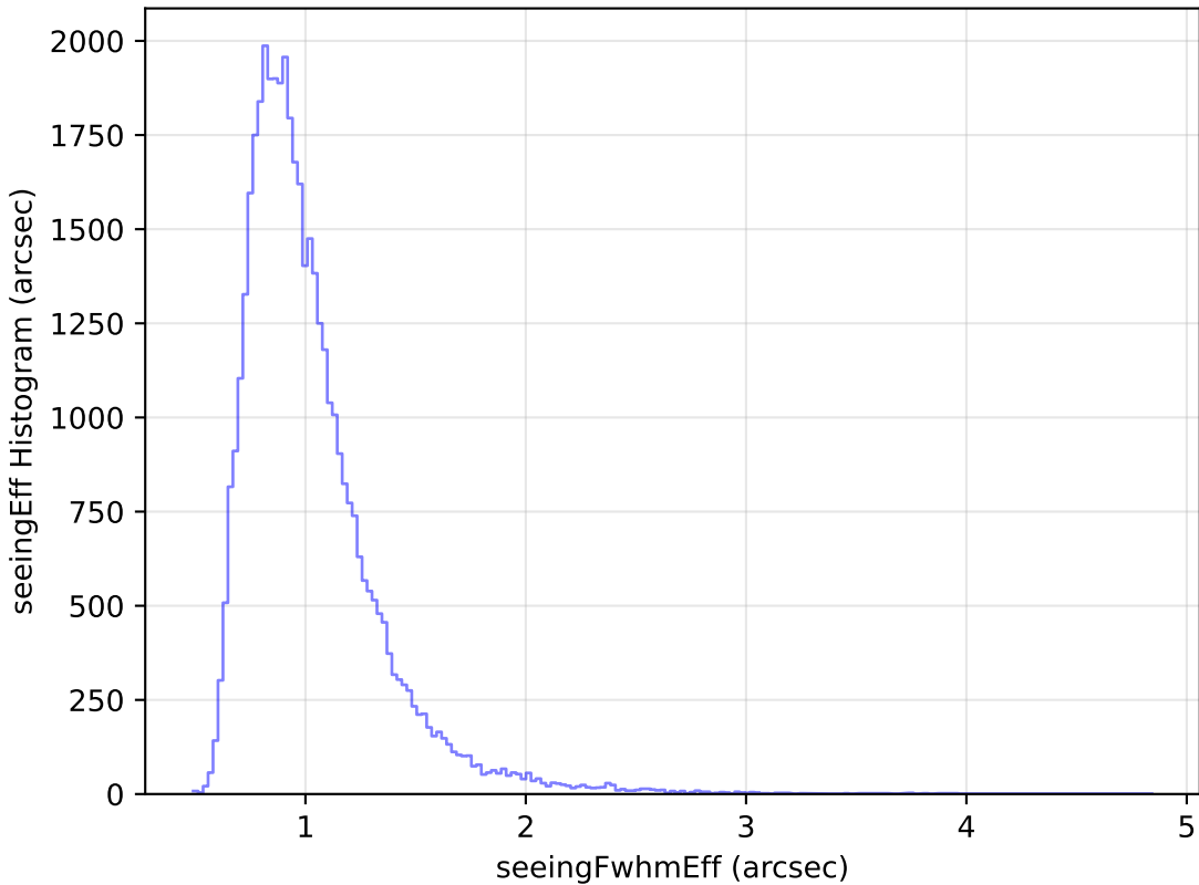
roll_pause_mjdp365_v3.4_10yrs Yr 1 z band: seeingEff Histogram
