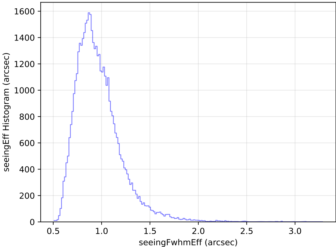
roll_pause_mjdp365_v3.4_10yrs Yr 1 y band: seeingEff Histogram
