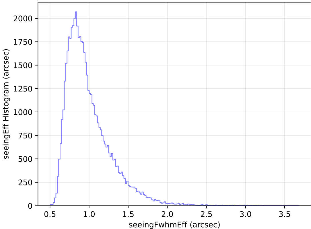
roll_pause_mjdp365_v3.4_10yrs Yr 1 i band: seeingEff Histogram
