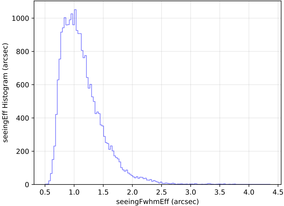
roll_pause_mjdp365_v3.4_10yrs Yr 1 g band: seeingEff Histogram
