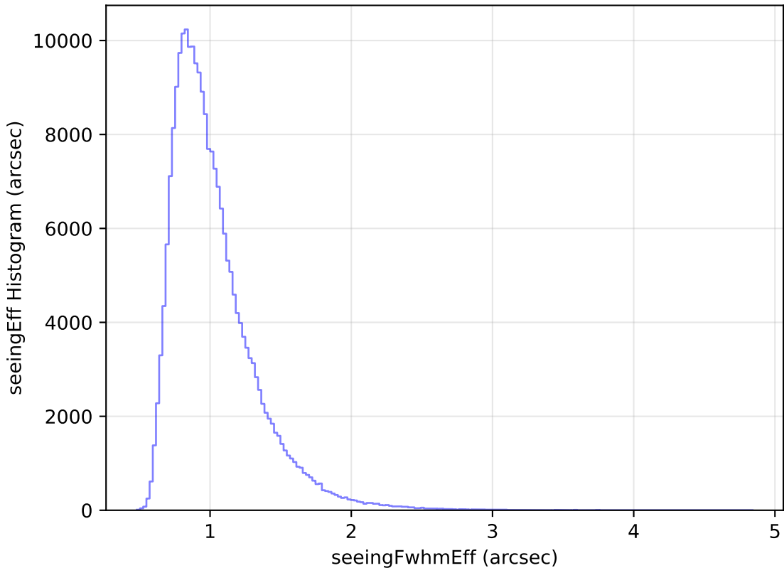
roll_pause_mjdp365_v3.4_10yrs Yr 1 all bands: seeingEff Histogram
