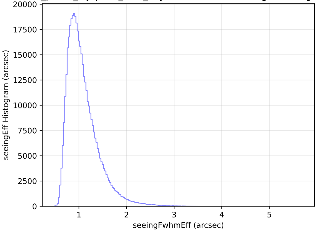
roll_pause_mjdp365_v3.4_10yrs WFD z band: seeingEff Histogram
