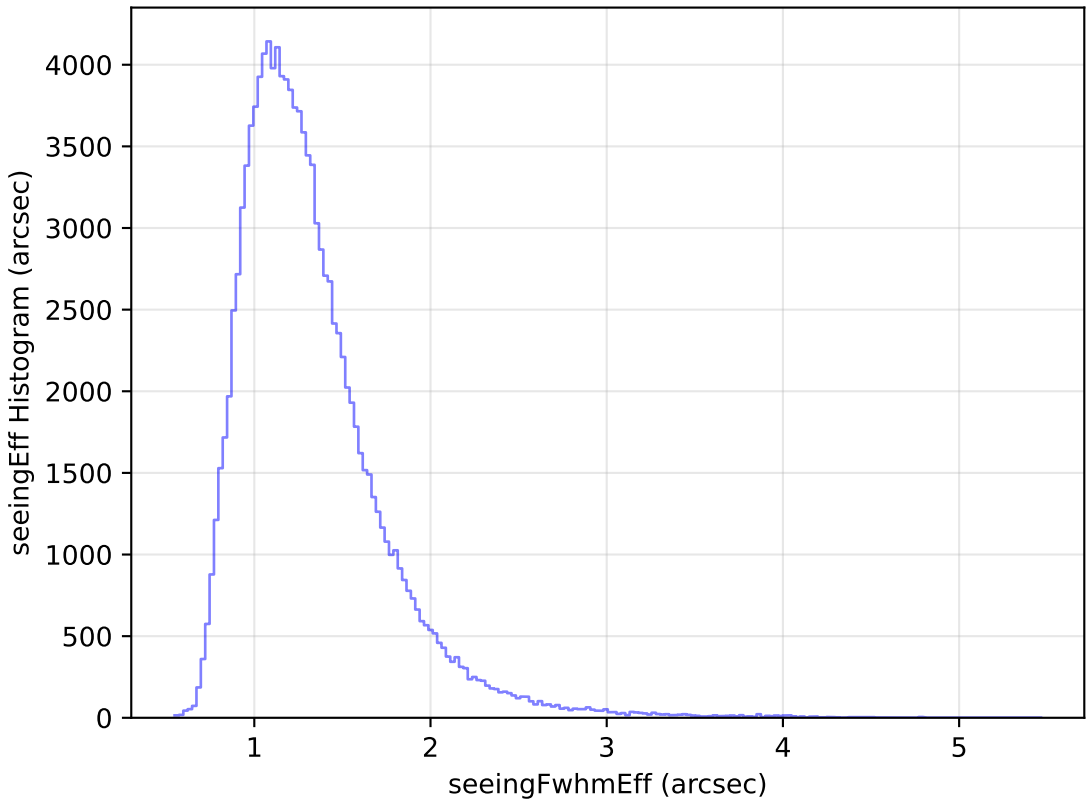
roll_pause_mjdp365_v3.4_10yrs WFD u band: seeingEff Histogram
