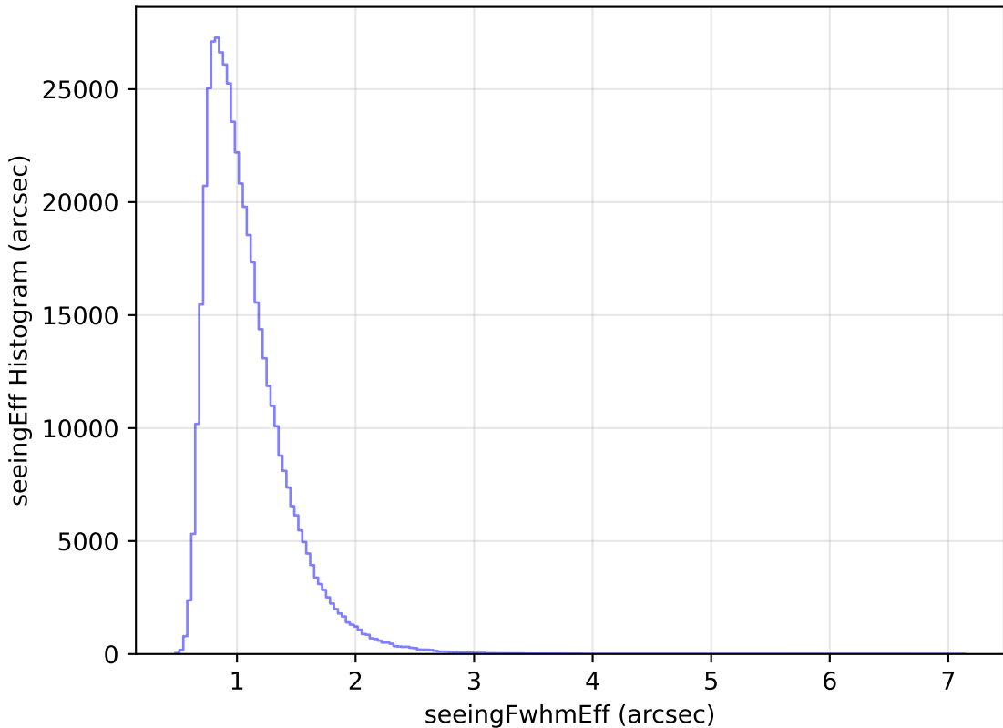
roll_pause_mjdp365_v3.4_10yrs WFD i band: seeingEff Histogram
