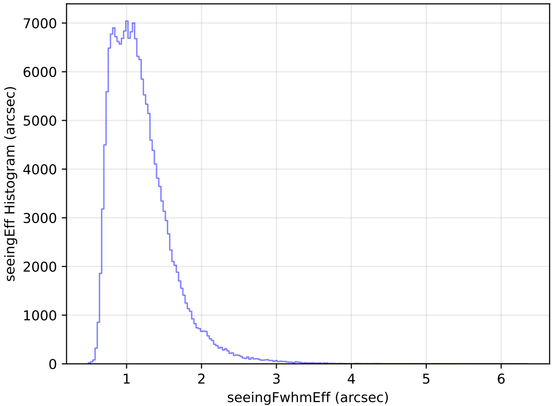
roll_pause_mjdp365_v3.4_10yrs WFD g band: seeingEff Histogram
