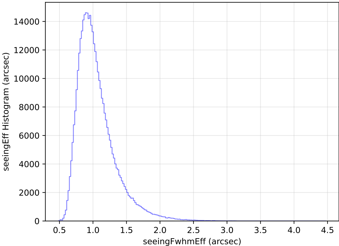
roll_pause_mjdp365_v3.4_10yrs All sky y band: seeingEff Histogram
