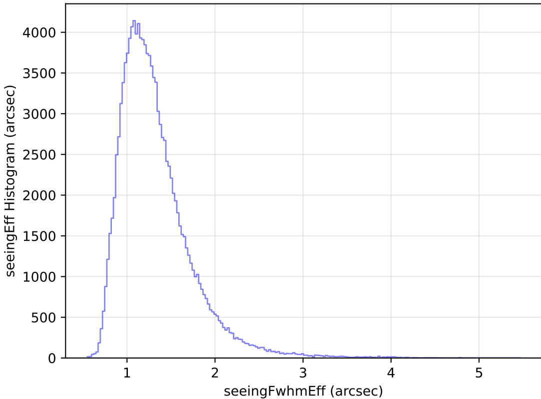
roll_pause_mjdp365_v3.4_10yrs All sky u band: seeingEff Histogram
