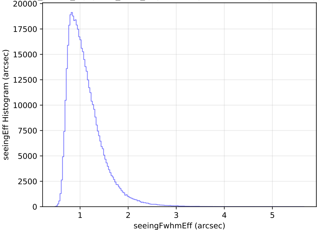
roll_pause_mjdp365_v3.4_10yrs All sky r band: seeingEff Histogram
