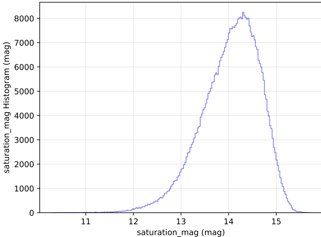
roll_pause_mjdp365_v3.4_10yrs WFD z band: saturation_mag Histogram
