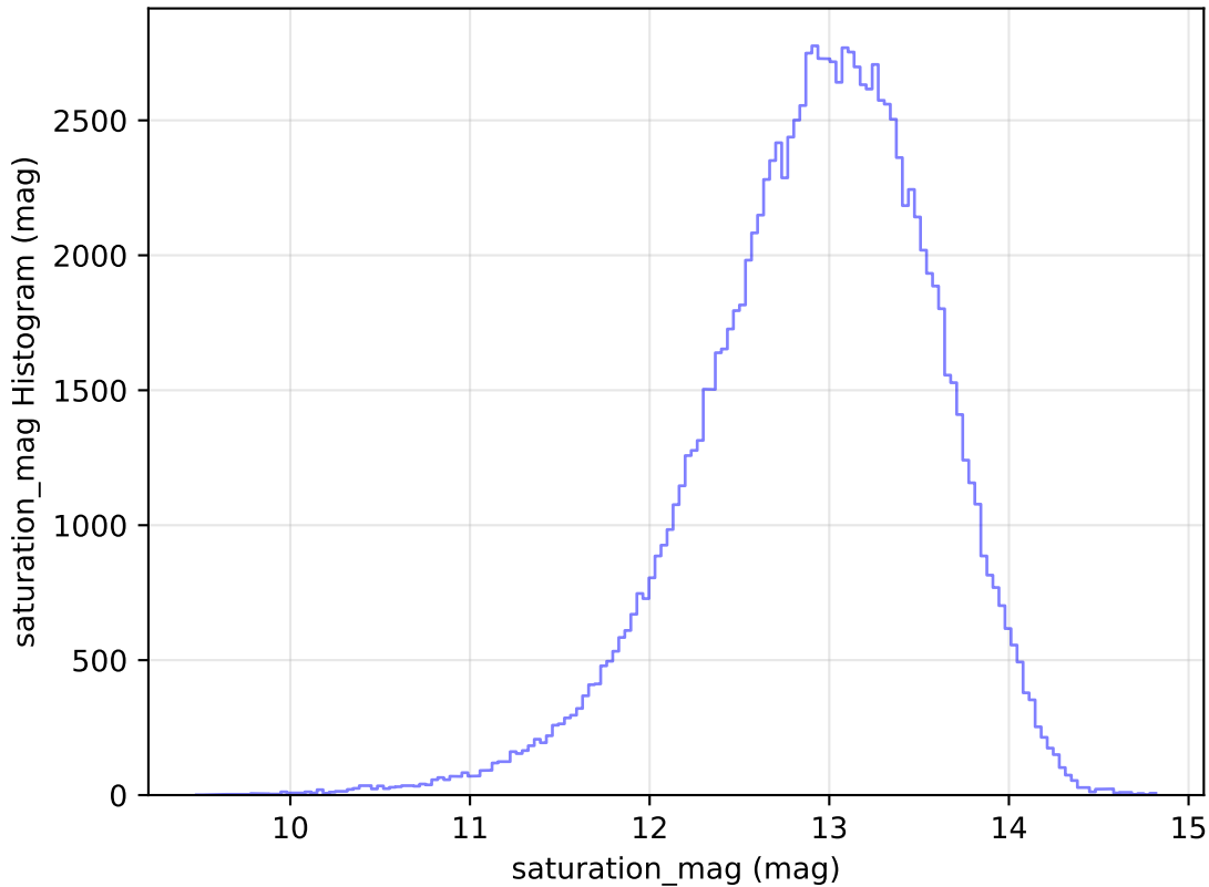
roll_pause_mjdp365_v3.4_10yrs WFD u band: saturation_mag Histogram
