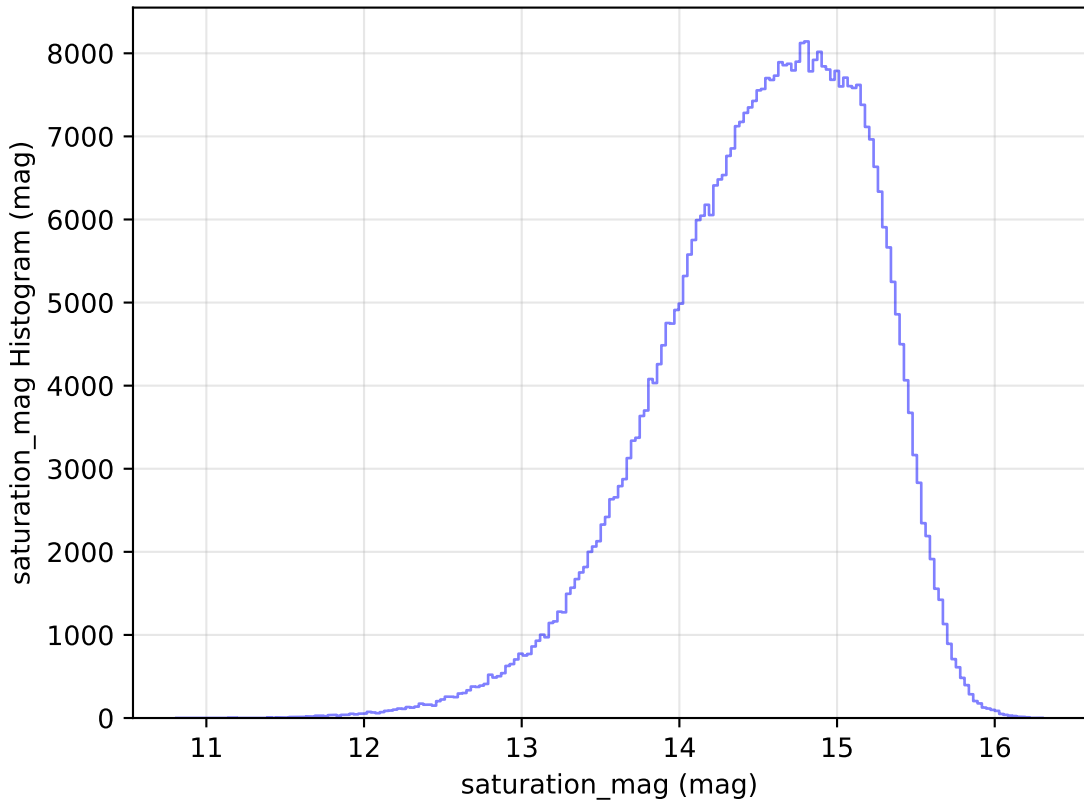
roll_pause_mjdp365_v3.4_10yrs WFD r band: saturation_mag Histogram
