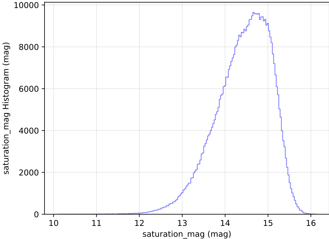
roll_pause_mjdp365_v3.4_10yrs WFD i band: saturation_mag Histogram
