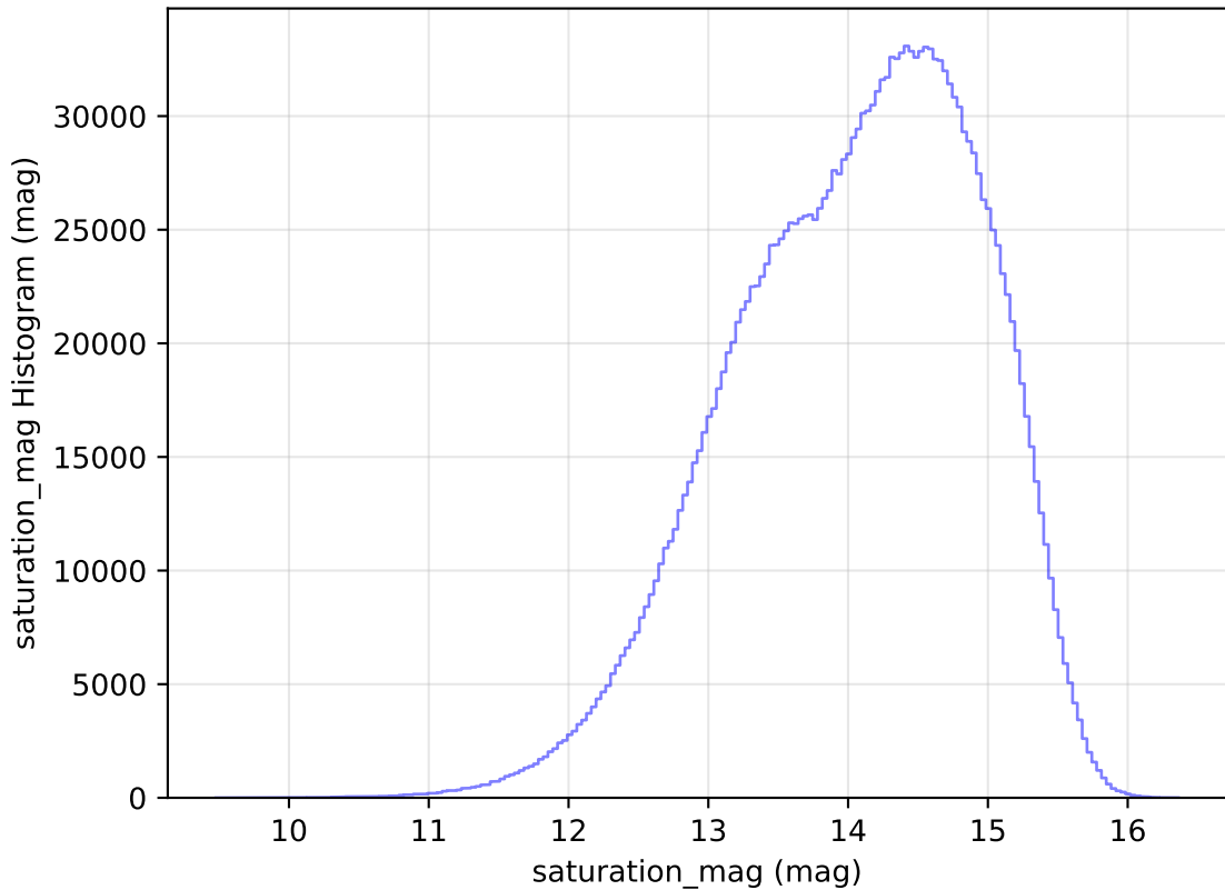
roll_pause_mjdp365_v3.4_10yrs WFD all bands: saturation_mag Histogram
