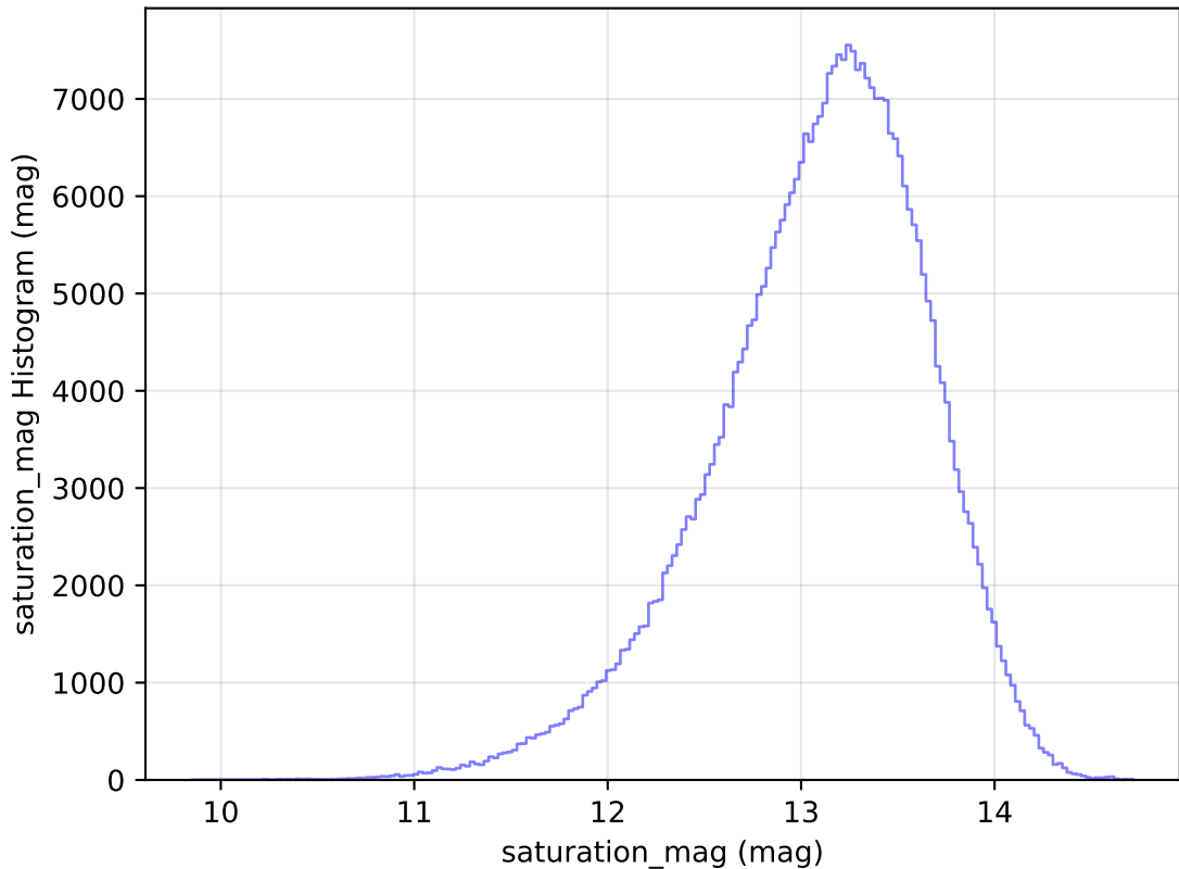
roll_pause_mjdp365_v3.4_10yrs All sky y band: saturation_mag Histogram
