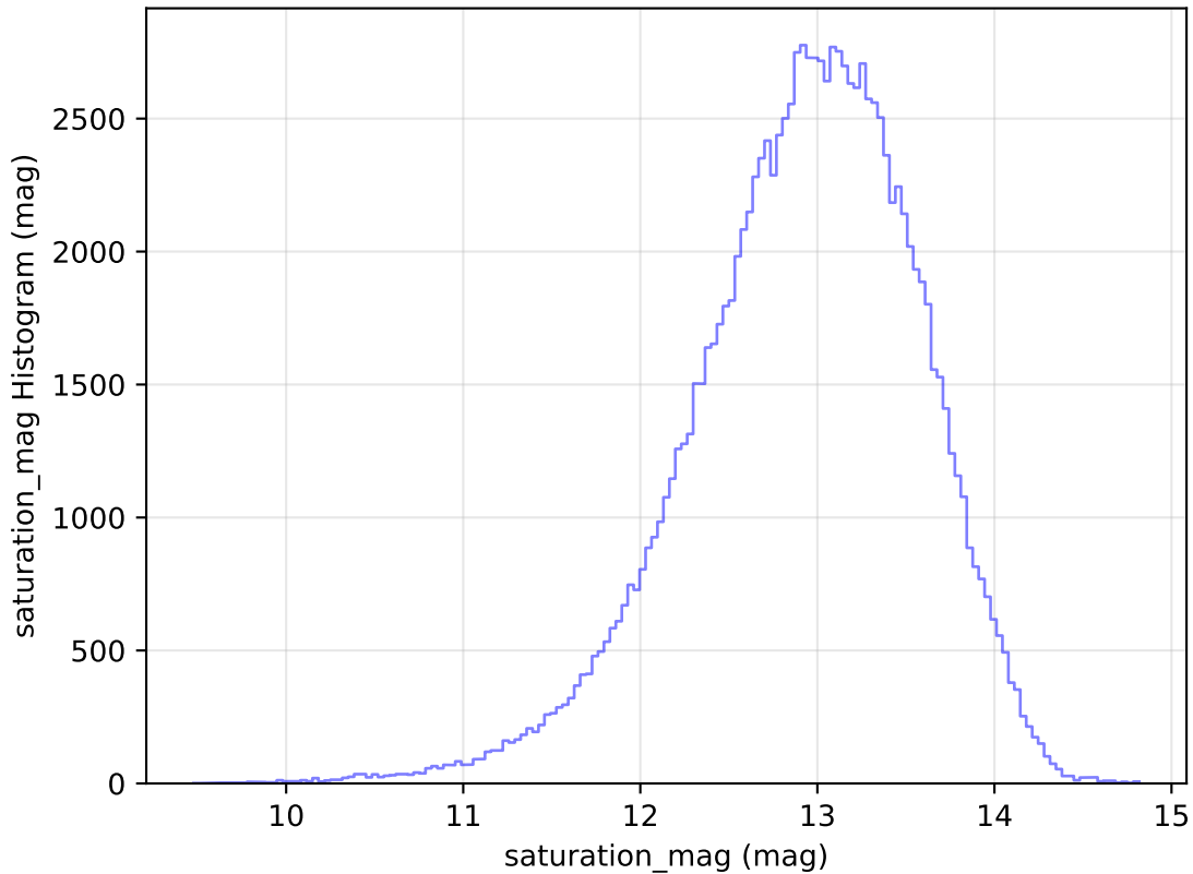
roll_pause_mjdp365_v3.4_10yrs All sky u band: saturation_mag Histogram
