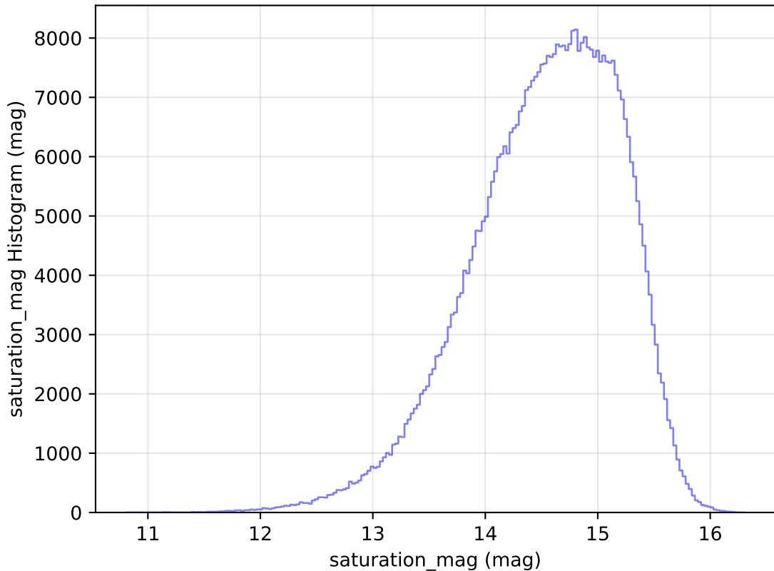
roll_pause_mjdp365_v3.4_10yrs All sky r band: saturation_mag Histogram
