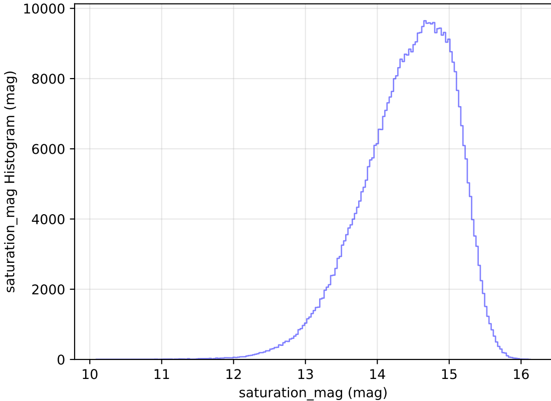
roll_pause_mjdp365_v3.4_10yrs All sky i band: saturation_mag Histogram
