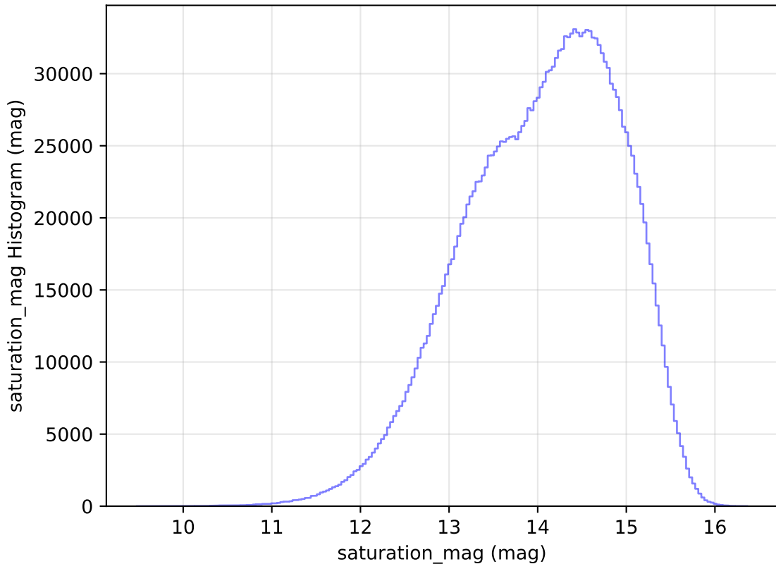
roll_pause_mjdp365_v3.4_10yrs All sky all bands: saturation_mag Histogram
