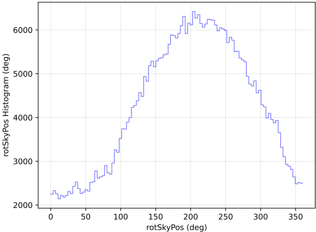
roll_pause_mjdp365_v3.4_10yrs WFD z band: rotSkyPos Histogram
