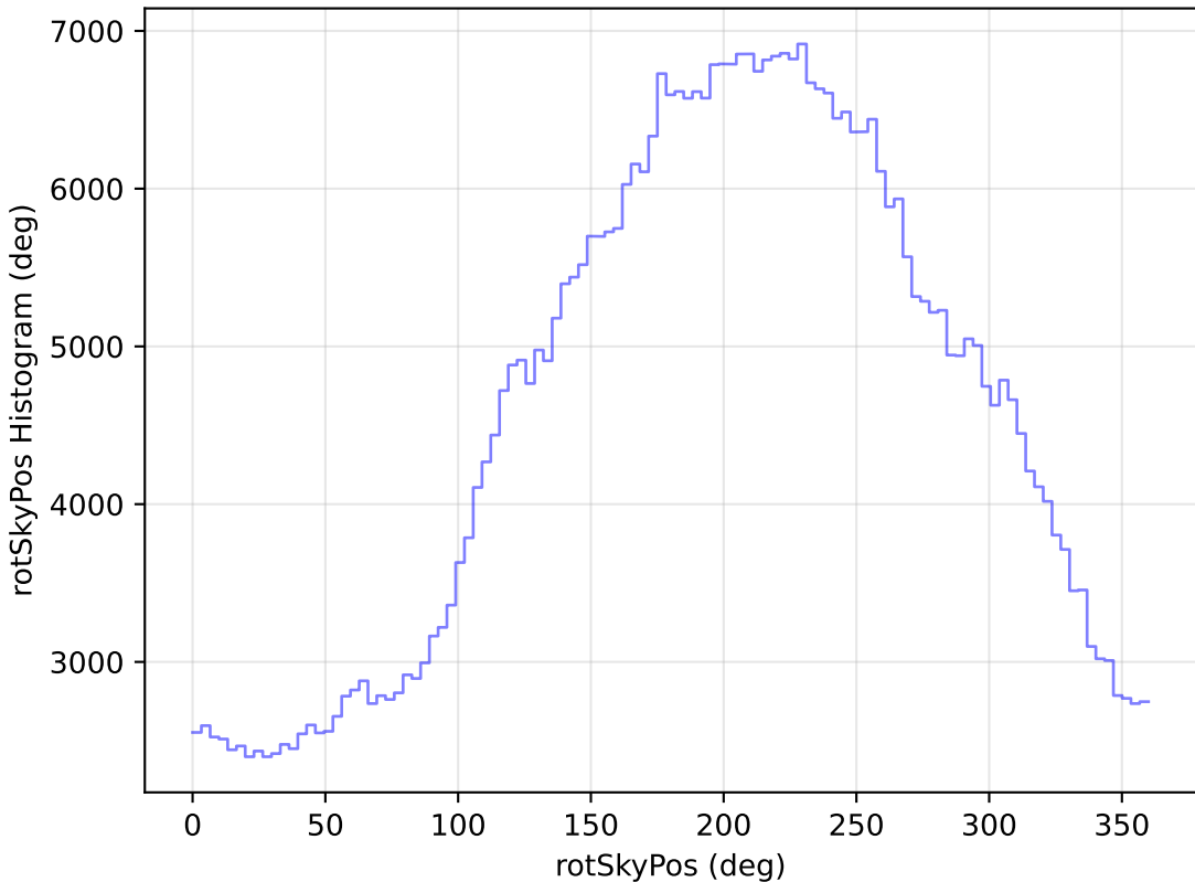
roll_pause_mjdp365_v3.4_10yrs WFD i band: rotSkyPos Histogram
