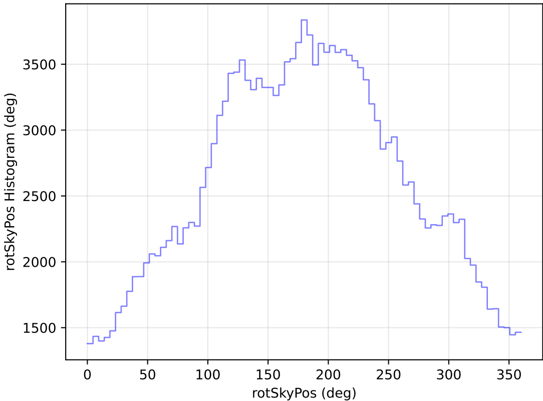
roll_pause_mjdp365_v3.4_10yrs WFD g band: rotSkyPos Histogram
