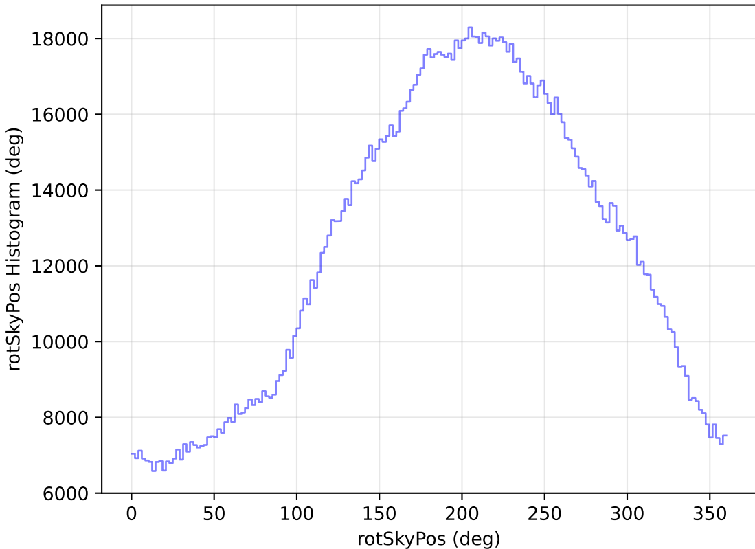
roll_pause_mjdp365_v3.4_10yrs WFD all bands: rotSkyPos Histogram
