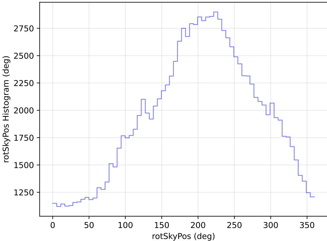
roll_pause_mjdp365_v3.4_10yrs All sky u band: rotSkyPos Histogram
