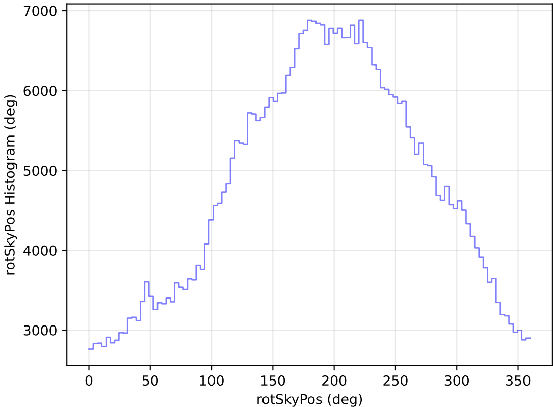
roll_pause_mjdp365_v3.4_10yrs All sky r band: rotSkyPos Histogram
