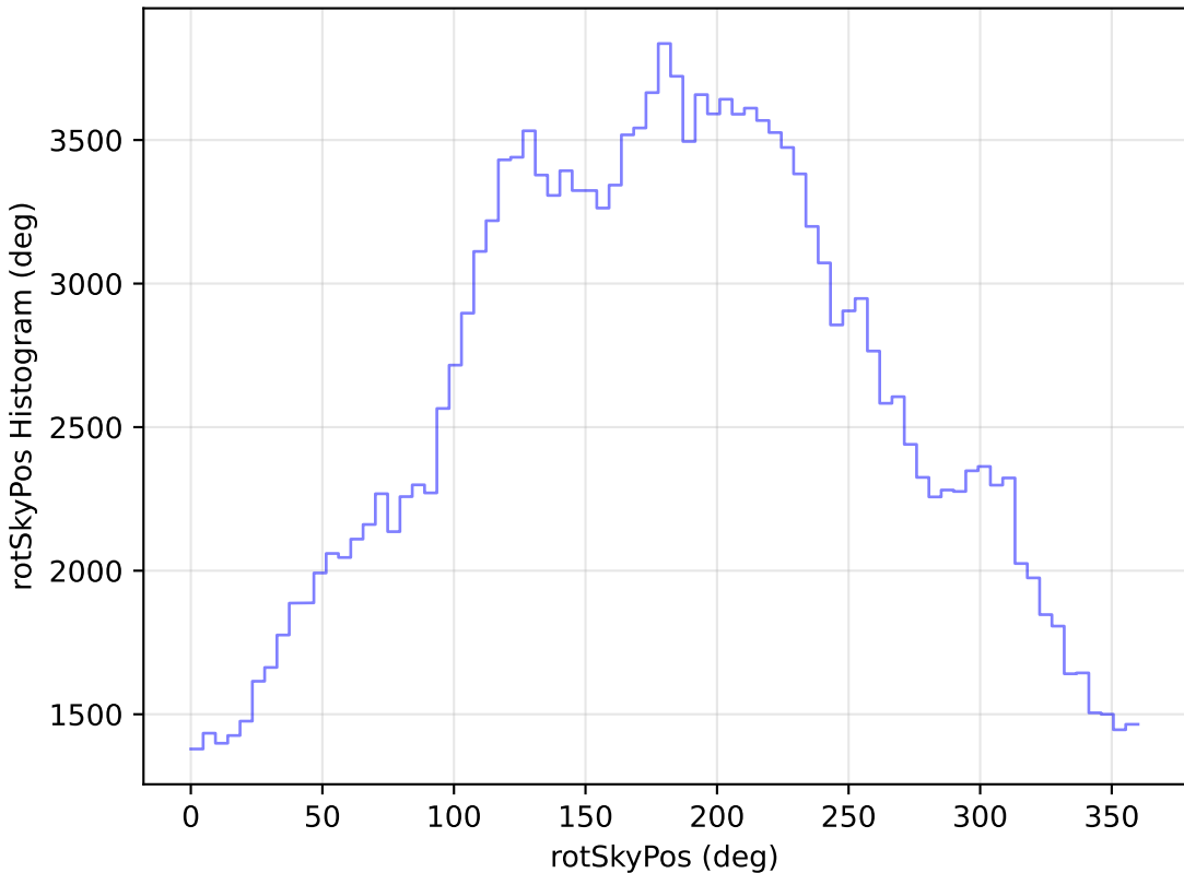
roll_pause_mjdp365_v3.4_10yrs All sky g band: rotSkyPos Histogram
