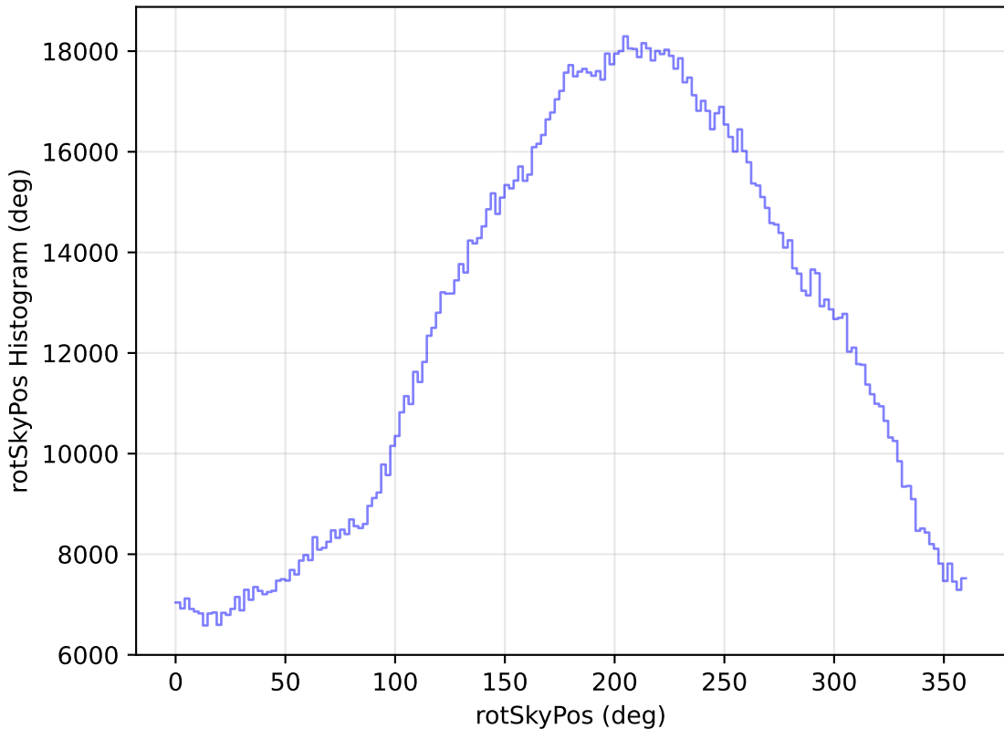
roll_pause_mjdp365_v3.4_10yrs All sky all bands: rotSkyPos Histogram
