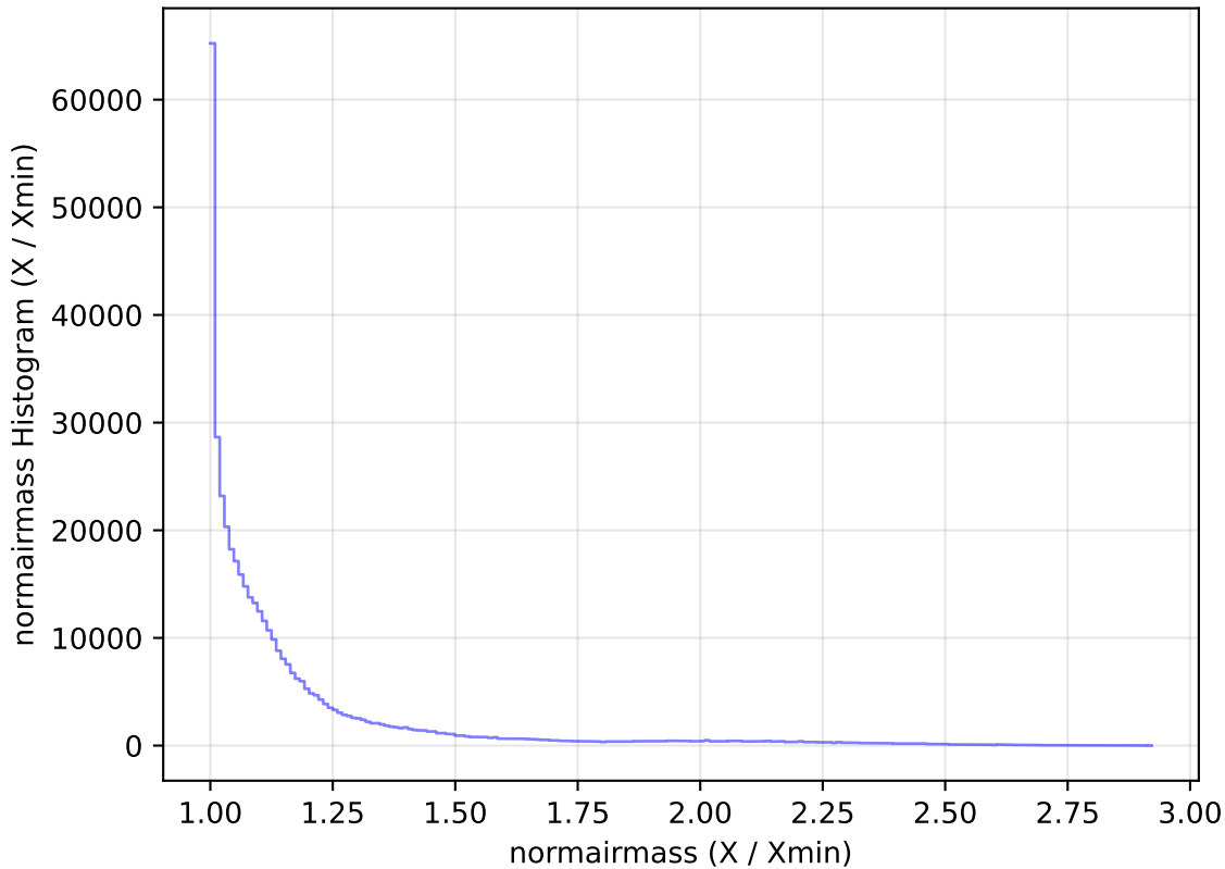
roll_pause_mjdp365_v3.4_10yrs WFD z band: normairmass Histogram
