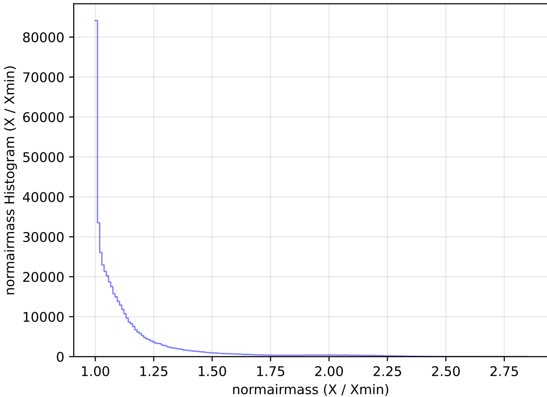
roll_pause_mjdp365_v3.4_10yrs WFD r band: normairmass Histogram
