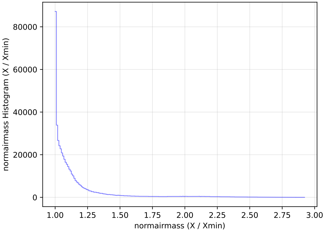
roll_pause_mjdp365_v3.4_10yrs WFD i band: normairmass Histogram
