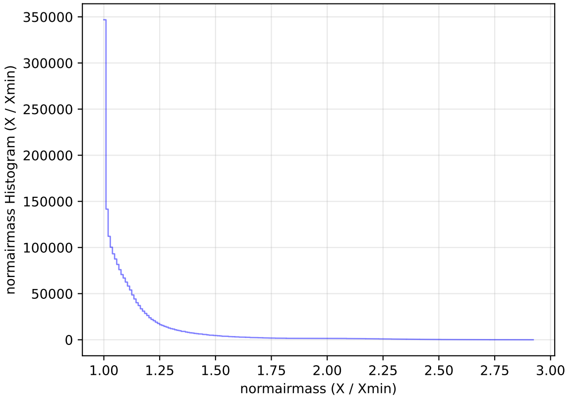
roll_pause_mjdp365_v3.4_10yrs WFD all bands: normairmass Histogram
