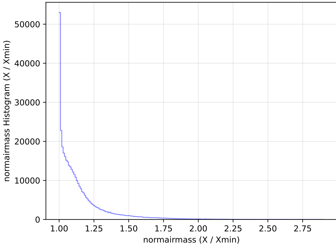
roll_pause_mjdp365_v3.4_10yrs All sky y band: normairmass Histogram
