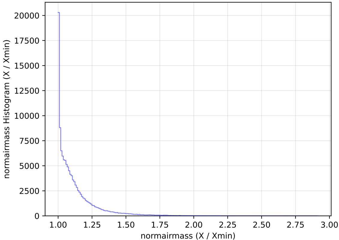
roll_pause_mjdp365_v3.4_10yrs All sky u band: normairmass Histogram
