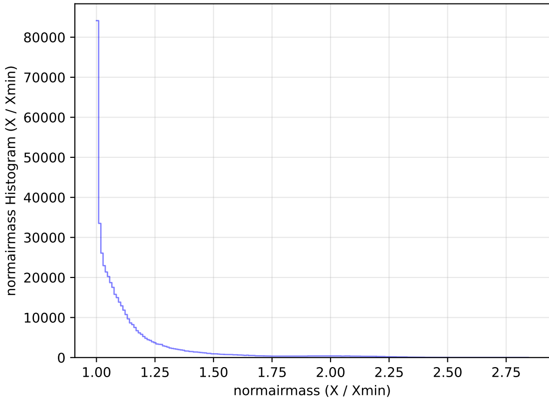
roll_pause_mjdp365_v3.4_10yrs All sky r band: normairmass Histogram
